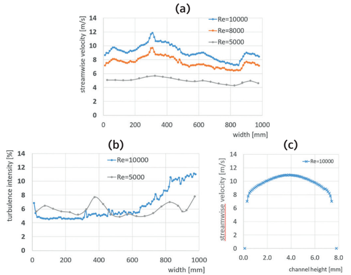
Figure 11 (a,b,c): Measurement results.
