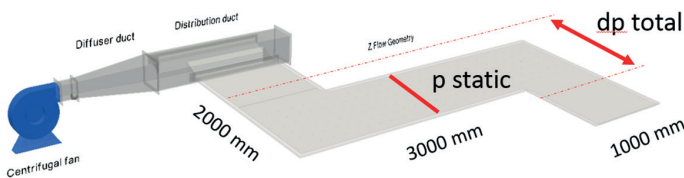
Figure 14: Position for static pressure measurement.
