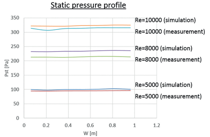
Figure 15: Comparison of measurement and simulation.
