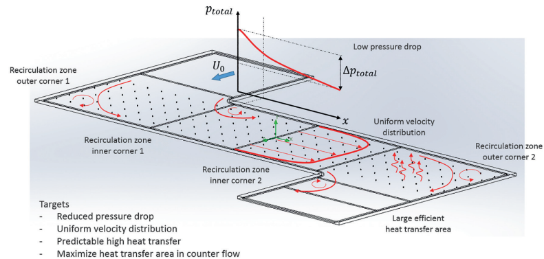
Figure 7: Flow conditions in a channel.
