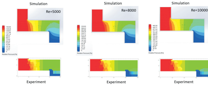
Figure 13: Comparison of test results with simulation results.
