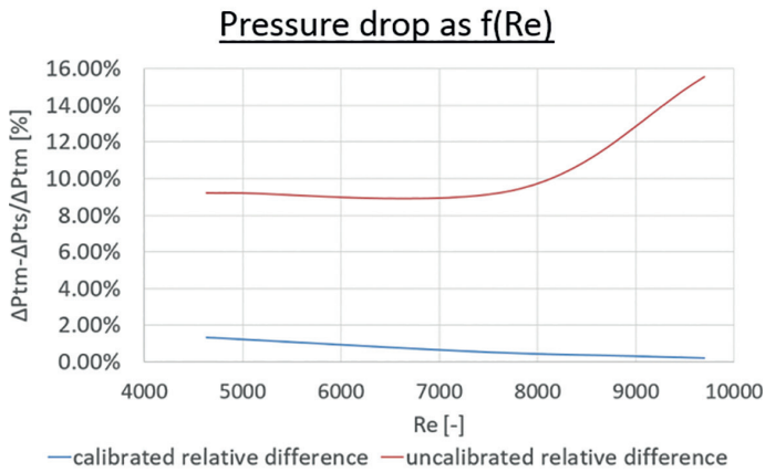
Figure 12: Deviation comparison for different boundary condition definitions.
