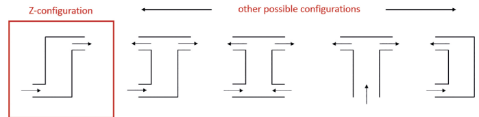
Figure 6: Possible configurations for gas flow arrangement.
