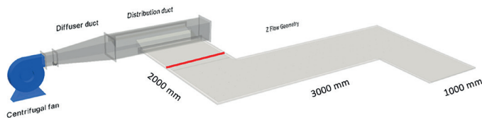
Figure 10: Physical flow model.
