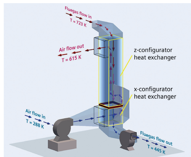
Figure 2: Basic design overview.
