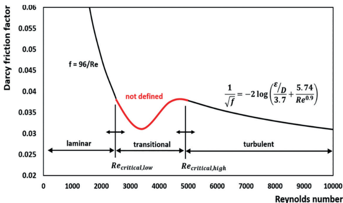
Figure 5: Reynolds number ranges.
