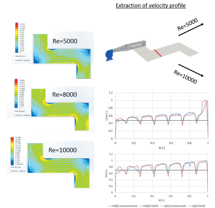
Figure 16: Comparison of the velocity profile.
