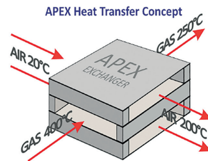
Figure 3: Principle heat exchange metal plates.
